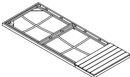
5 Seat Frame (Left) Qty 1 (1830 x 55mm)(720 x 55mm)
