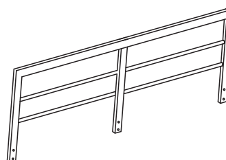
4 Backrest Qty 2 (1420 x 20mm)(462 x 20mm)
