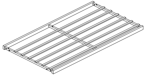
2 Seat frame Qty 2 (133x75x5 cm)
