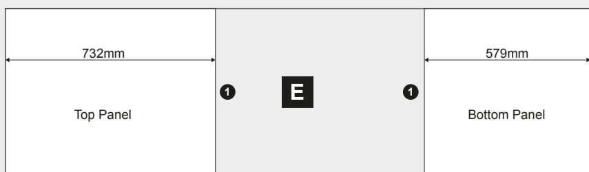
Single Oven Appliance Unit
