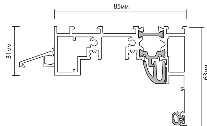
FRAME HEAD
