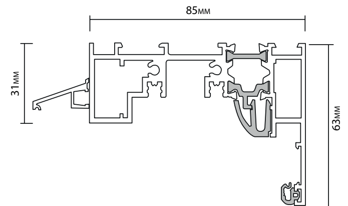
FRAME HEAD
