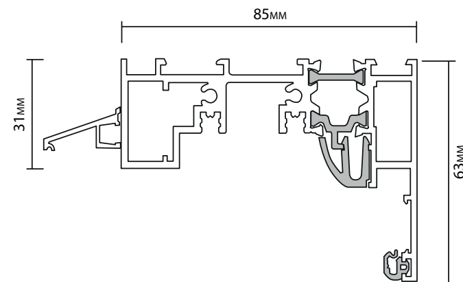
FRAME HEAD
