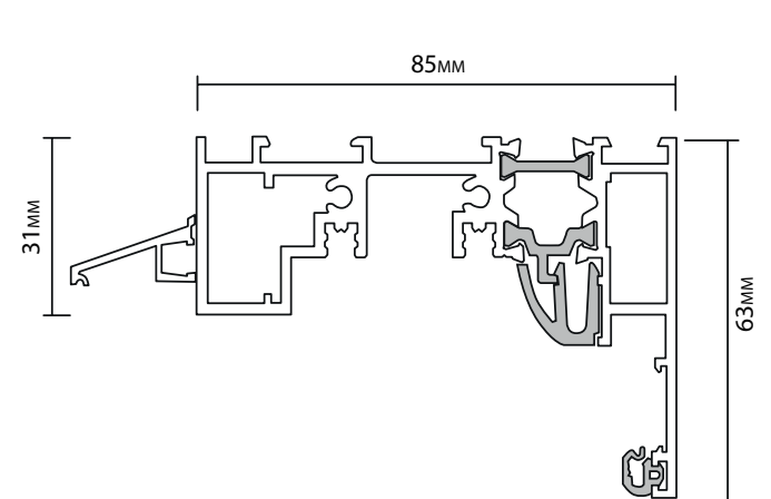
FRAME HEAD
