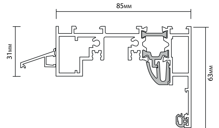
FRAME HEAD
