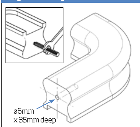
Fig.31 - Fitting
