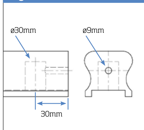
Fig.32 - Handrail
