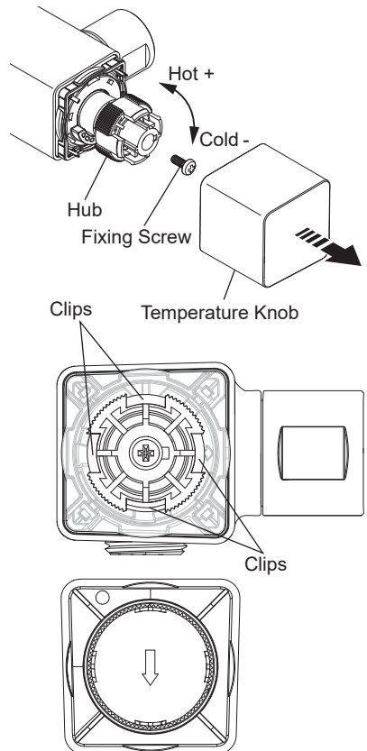
Inside View of Temperature Knob
