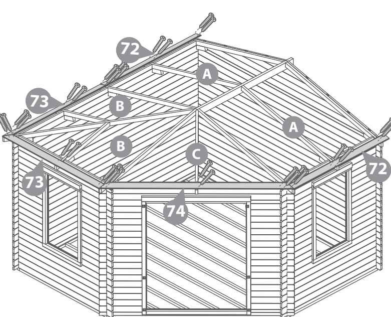
Roof Assembly 2
