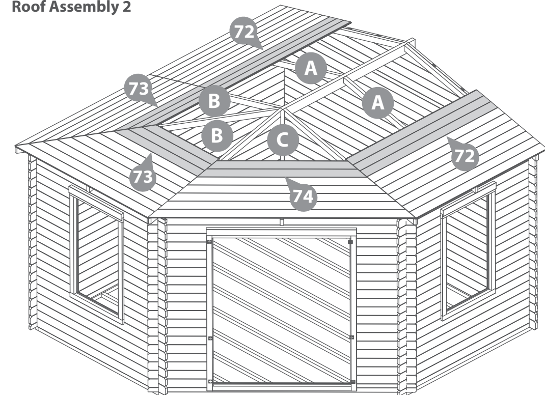
Roof Assembly 2
