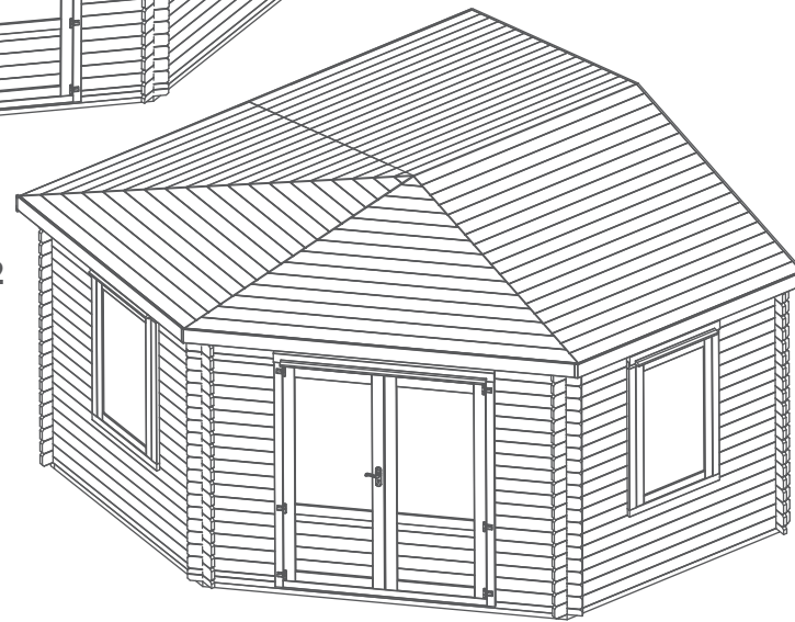
Roof Assembly 2
