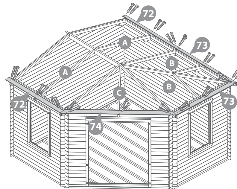
Roof Assembly 1
