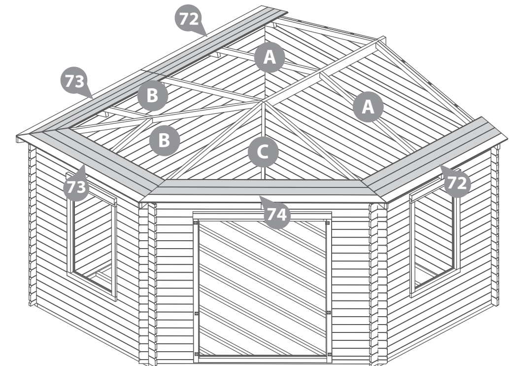
Roof Assembly 2
