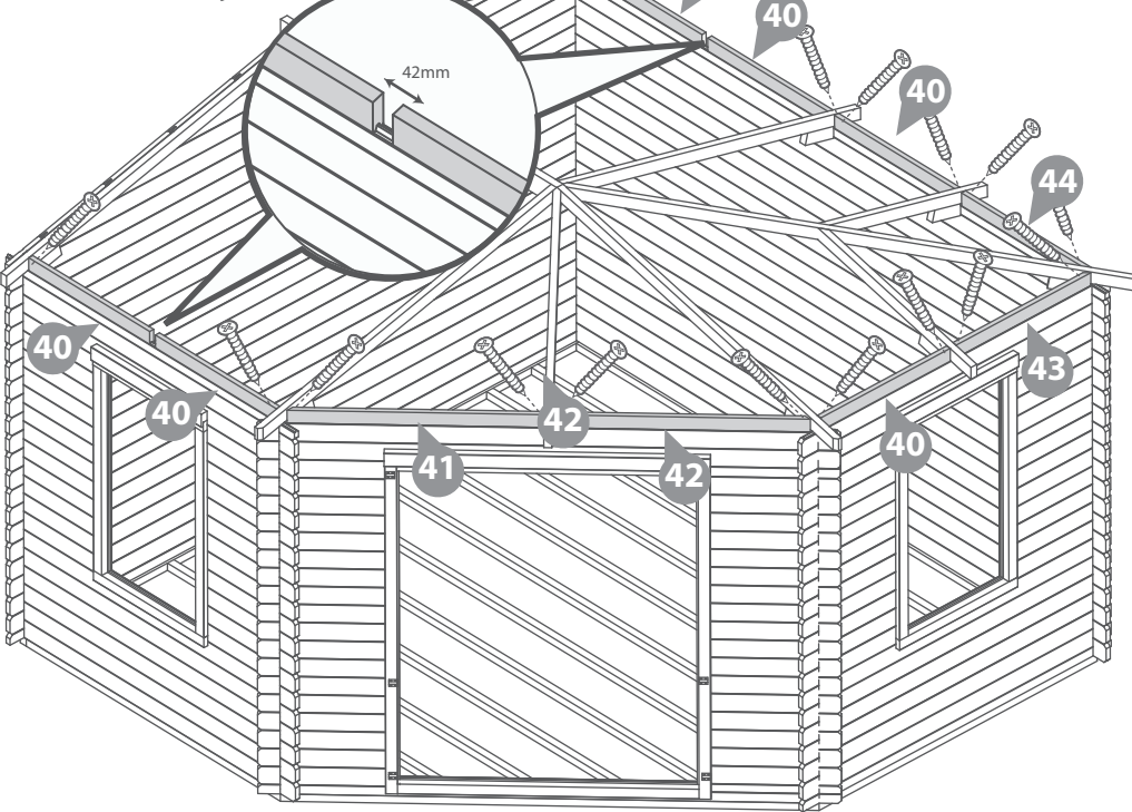
Roof Assembly 1
