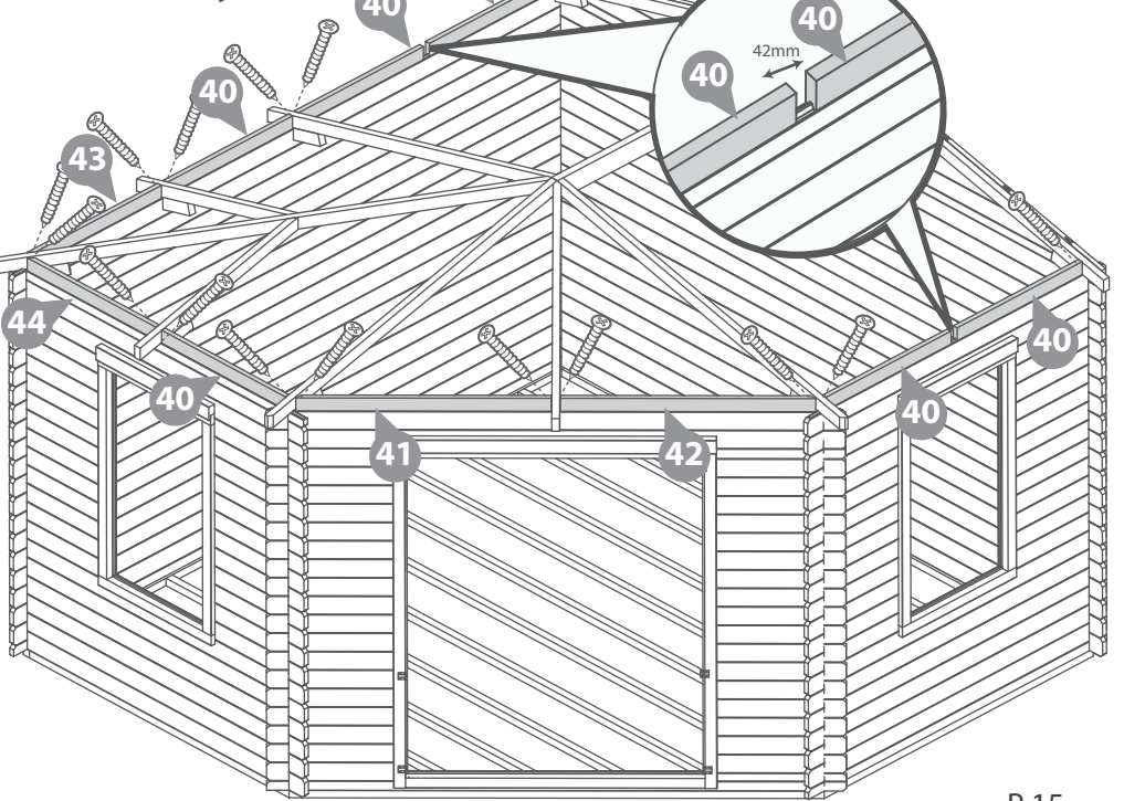
Roof Assembly 2
