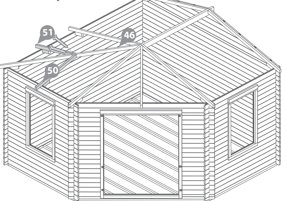
Roof Assembly 2
