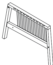
5 Leg Frame (Right) Qty 1 (585x83mm) (880x83mm)
