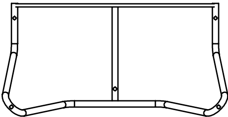
3 Leg frame (back) Qty1 (78x77x36cm)
