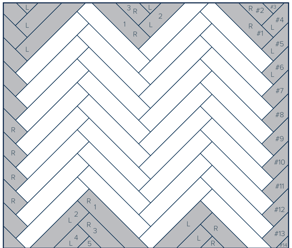
FIGURE 6 : Completing cut sections of the floor
