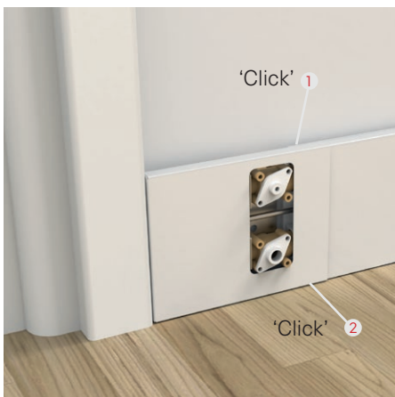
TRV Cover 1. Clip on Top 2. Swing and clip under
