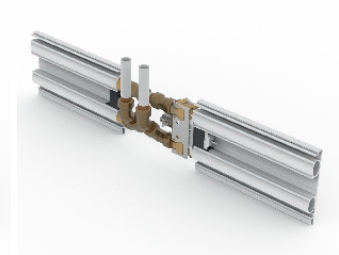
Pipes dropping from above (Solid wall)
