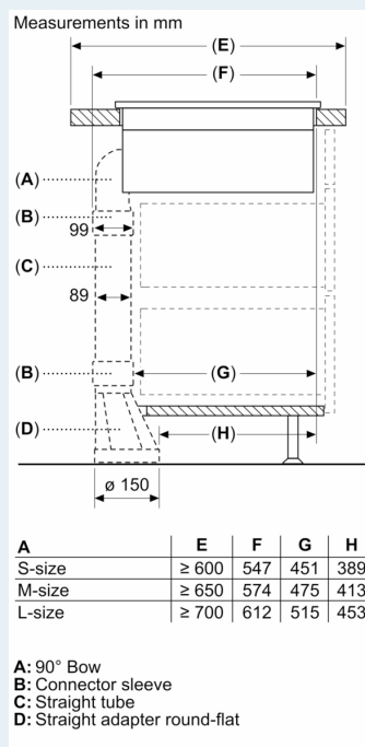
measurements in mm Front view
