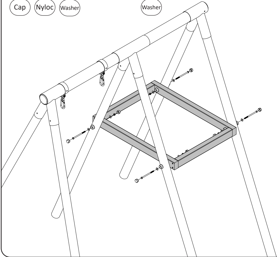
M8 x 135mm Hex Bolt (4)
