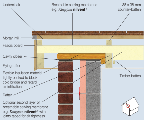
Figure 7c – Eaves Detail
