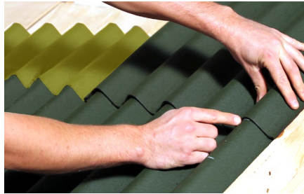
1 corrugation lap
